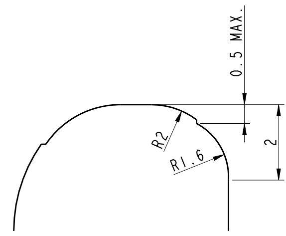
ENTRANCE BORE DETAIL SCALE 10:1
