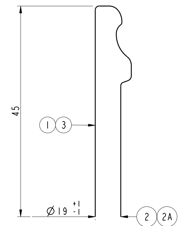
BORE DETAIL SCALE 2/1
